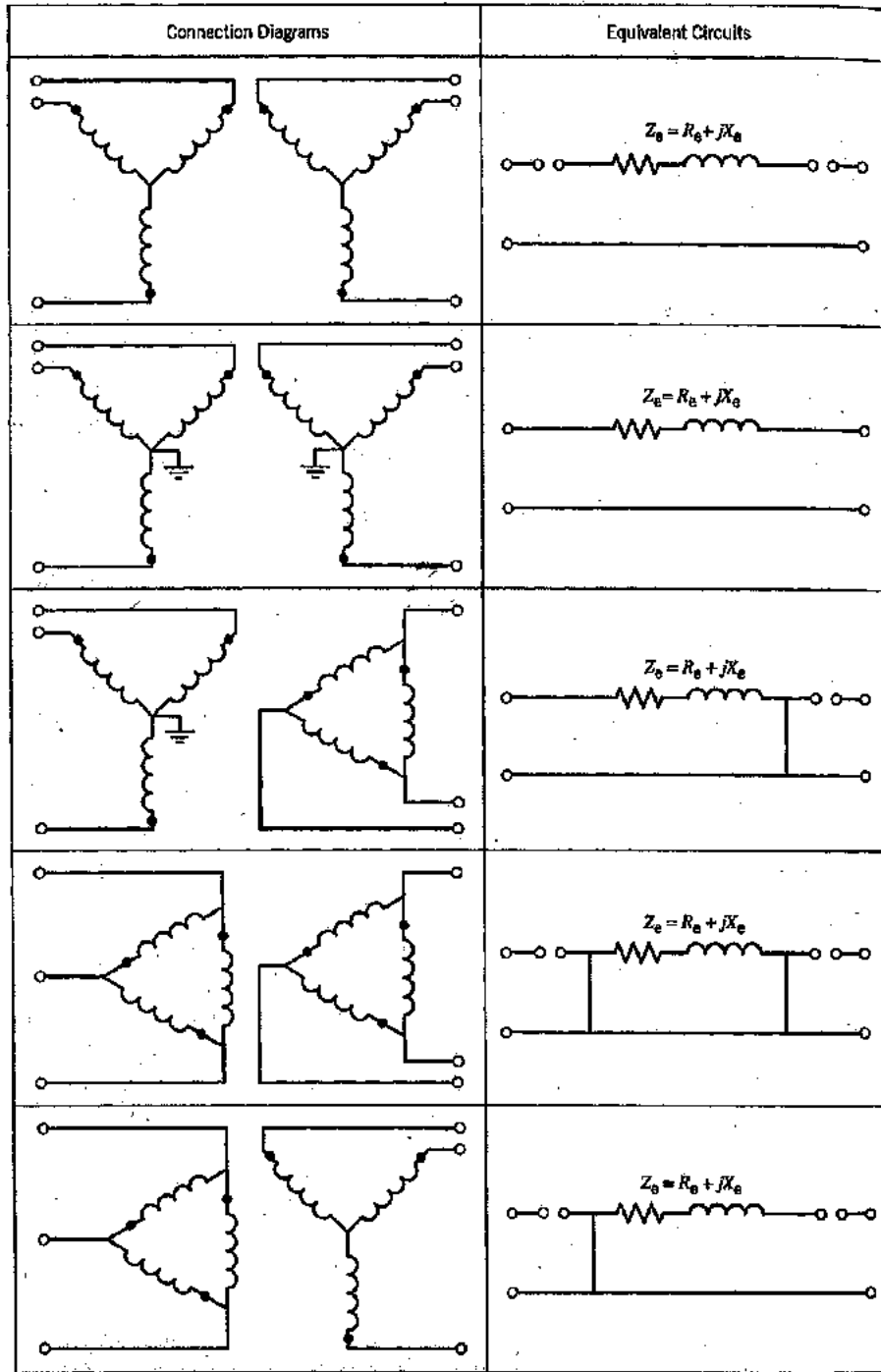
FIGURE 11.4 Zero-sequence equivalent circuits of three-phase transformer banks.
