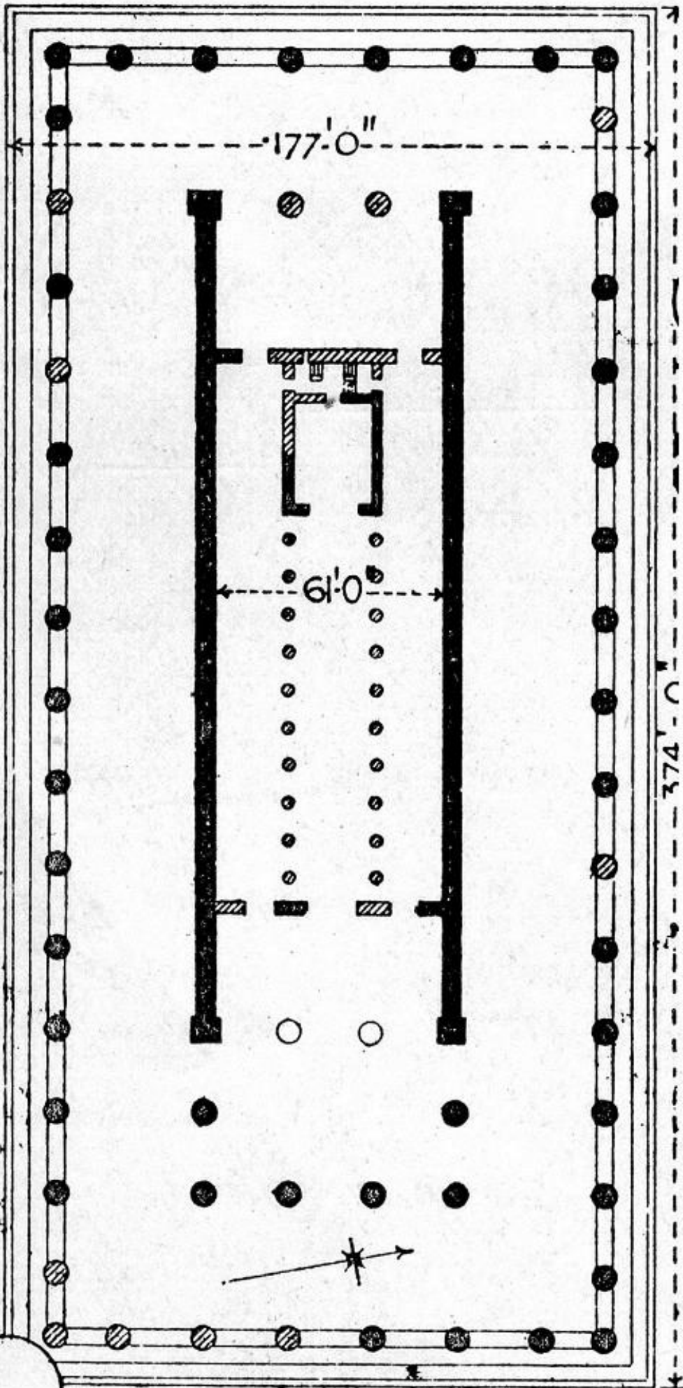
G. TEMPLE: SELINUS PSEUDODIPTERAL OCTASTYLE (DORIC)
